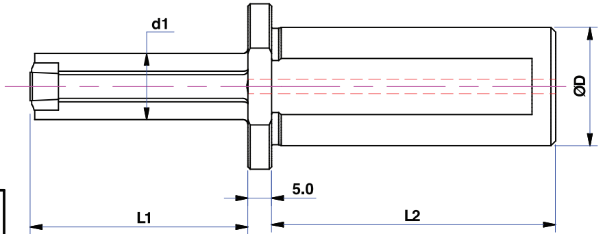
Holder dimensions
